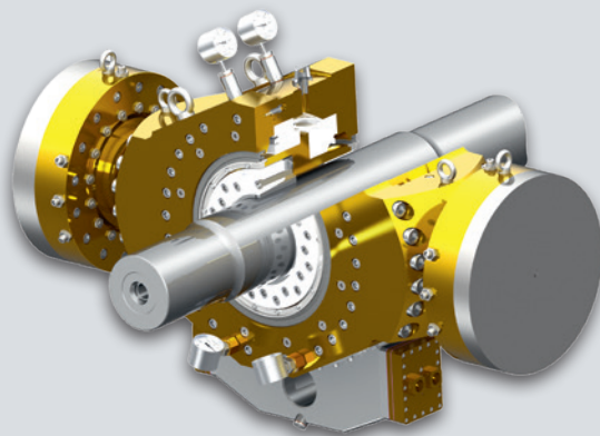
Piening - Drucklager
